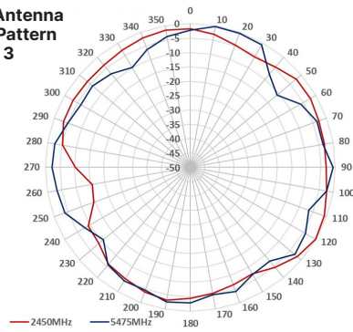
Internal Antenna H-Plane Pattern Radio 2
